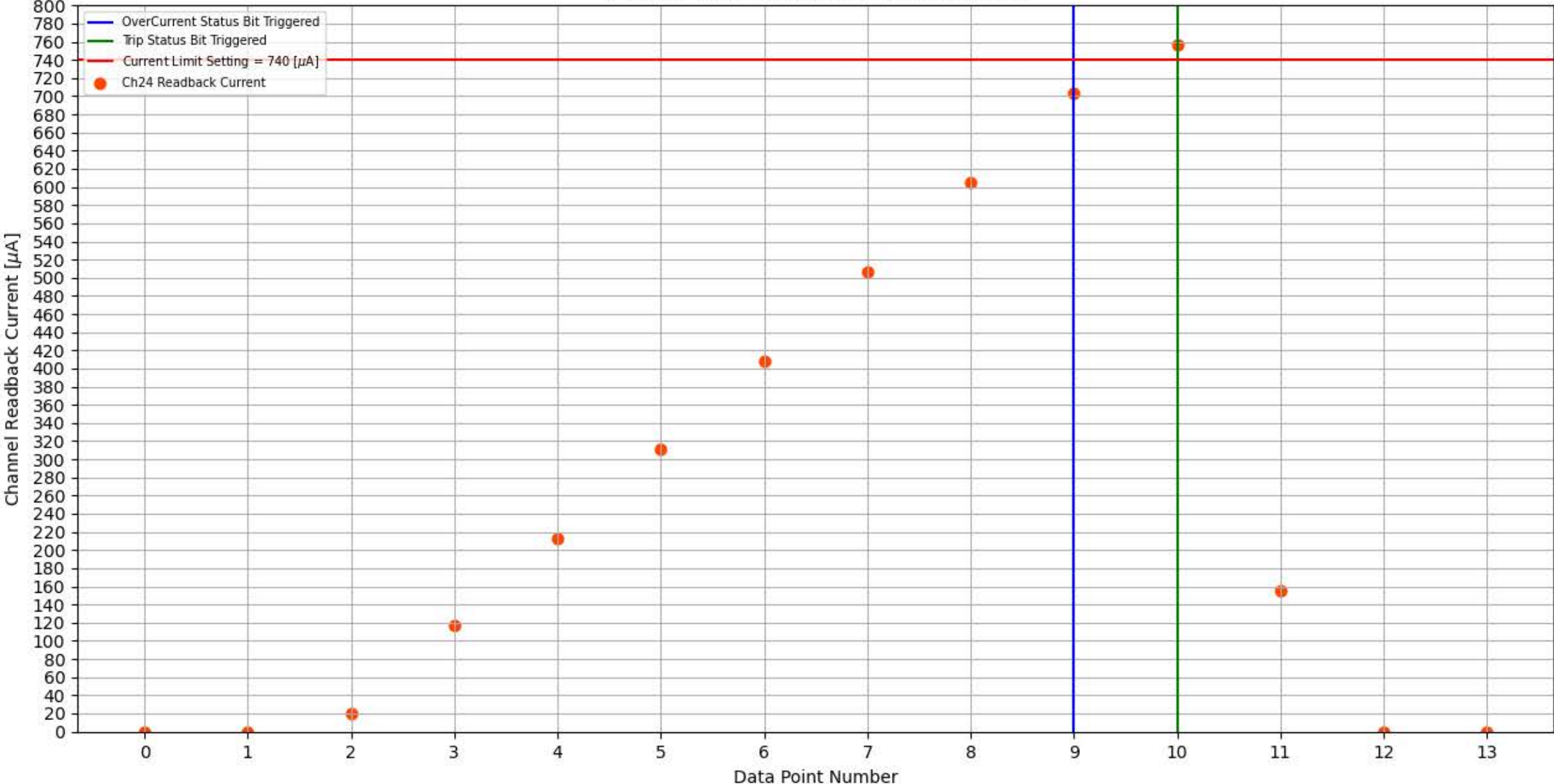
Module 256, Slot 3, Channel 24 Trip Test
