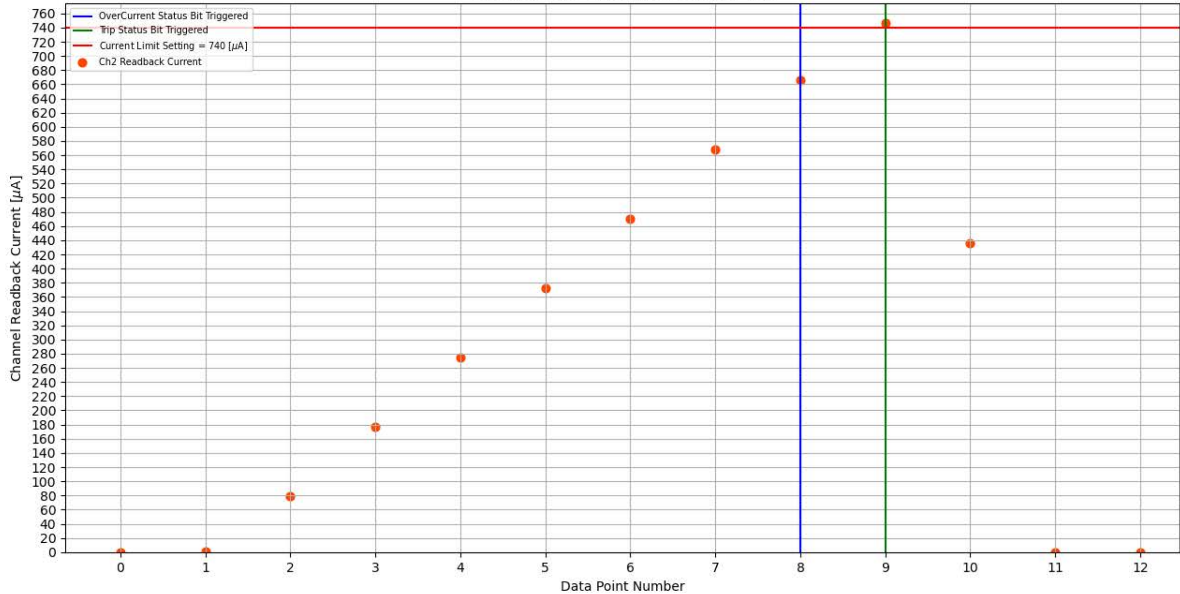
Module 256, Slot 3, Channel 2 Trip Test
