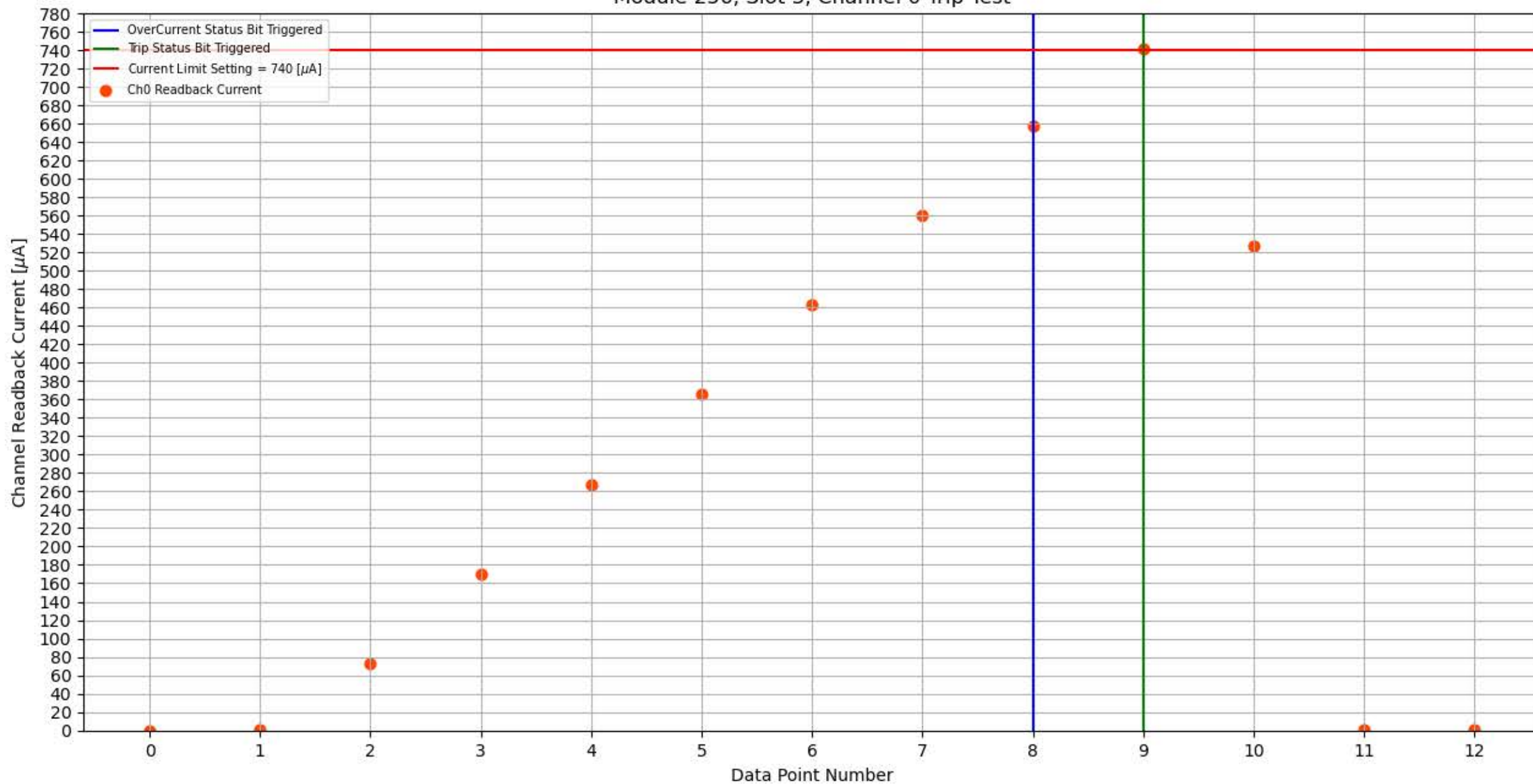
Module 256, Slot 3, Channel 0 Trip Test
