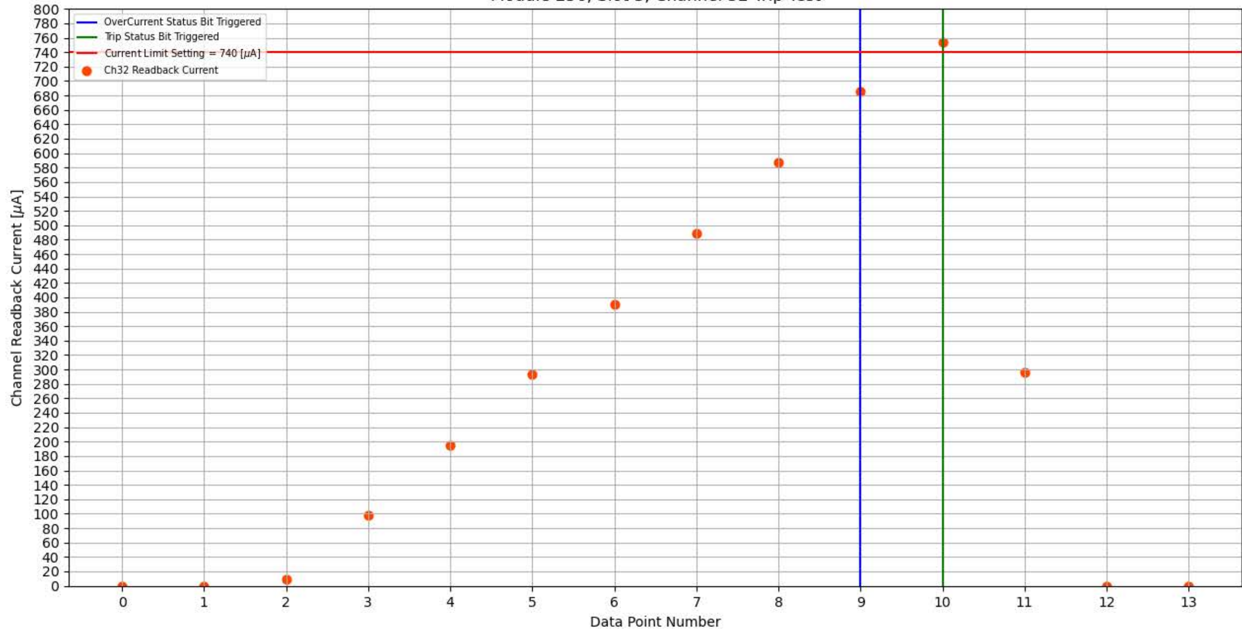
Module 256, Slot 3, Channel 32 Trip Test
