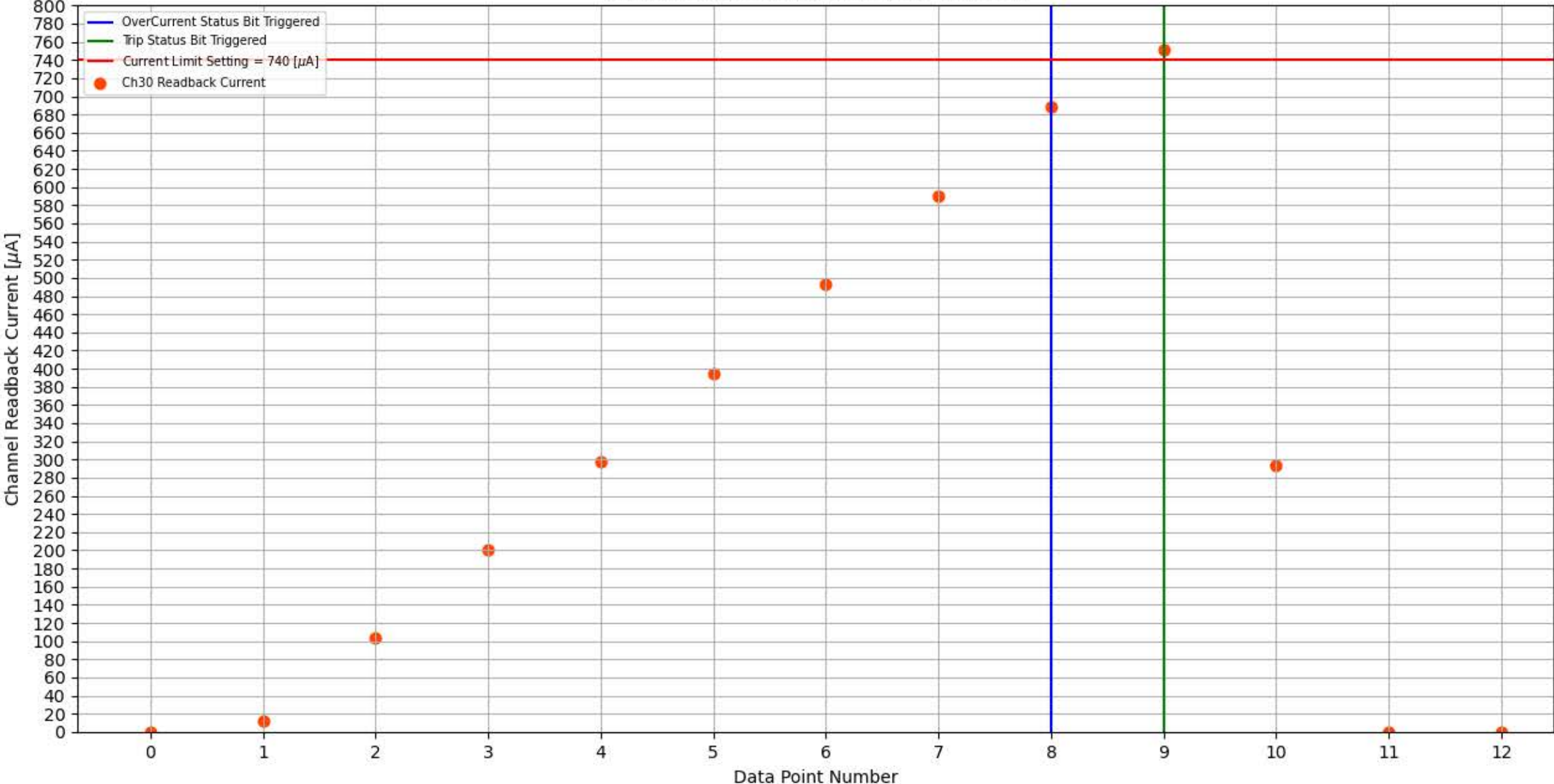
Module 256, Slot 3, Channel 30 Trip Test
