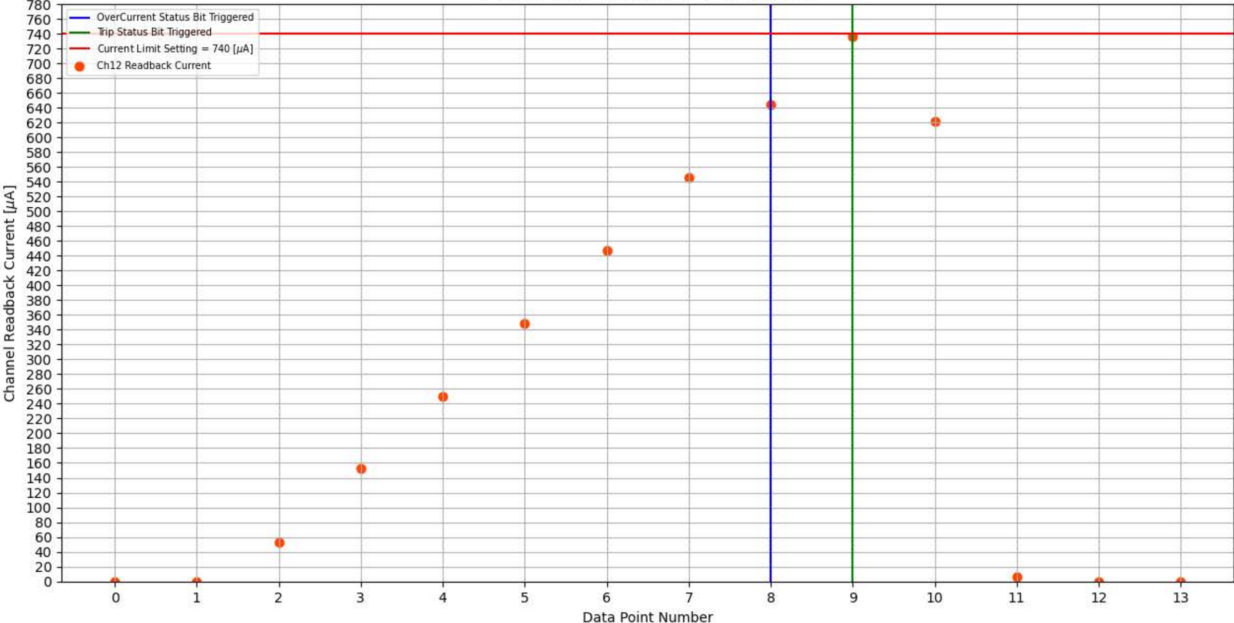
Module 256, Slot 3, Channel 12 Trip Test
