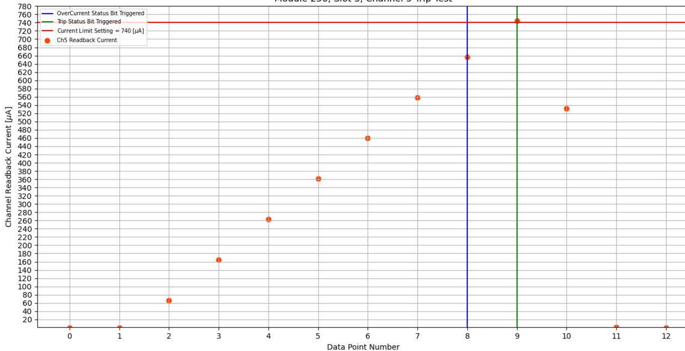
Module 256, Slot 3, Channel 5 Trip Test
