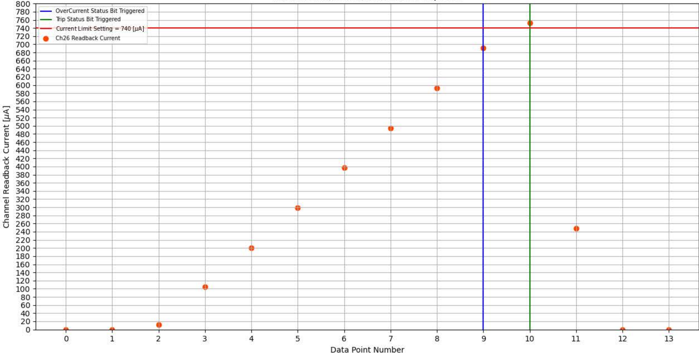
Module 256, Slot 3, Channel 26 Trip Test
