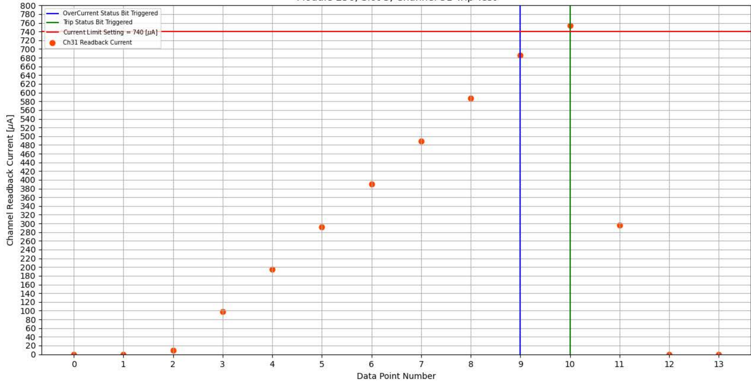
Module 256, Slot 3, Channel 31 Trip Test
