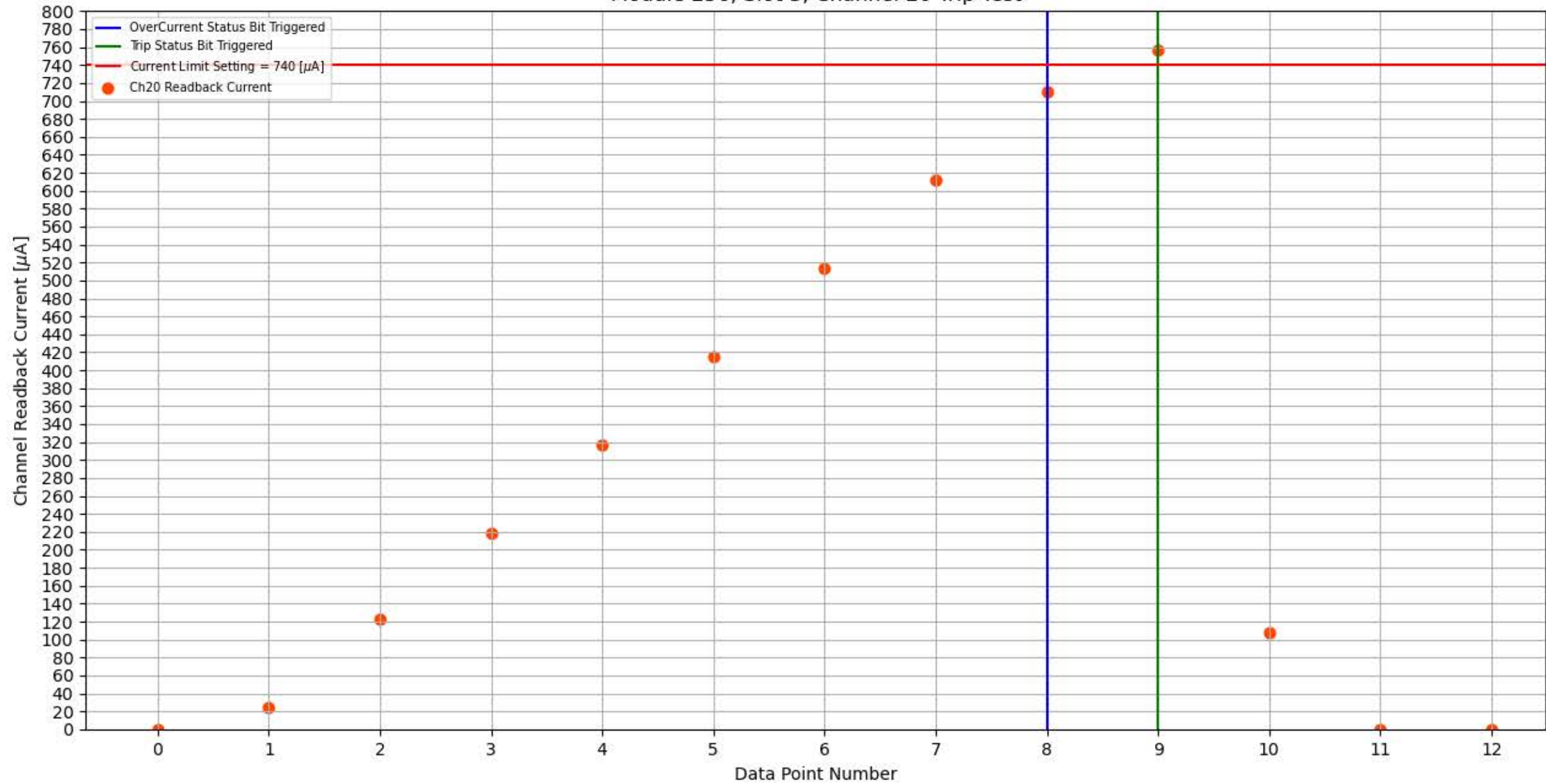
Module 256, Slot 3, Channel 20 Trip Test
