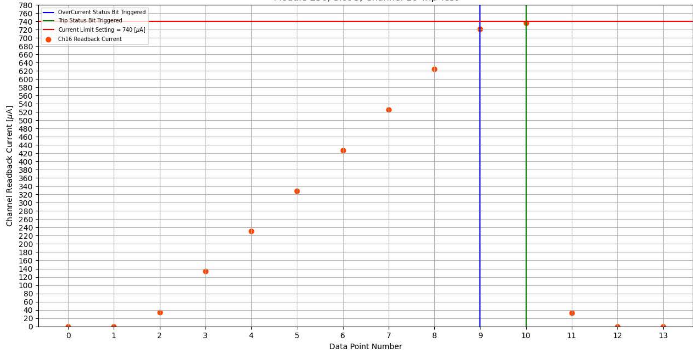
Module 256, Slot 3, Channel 16 Trip Test
