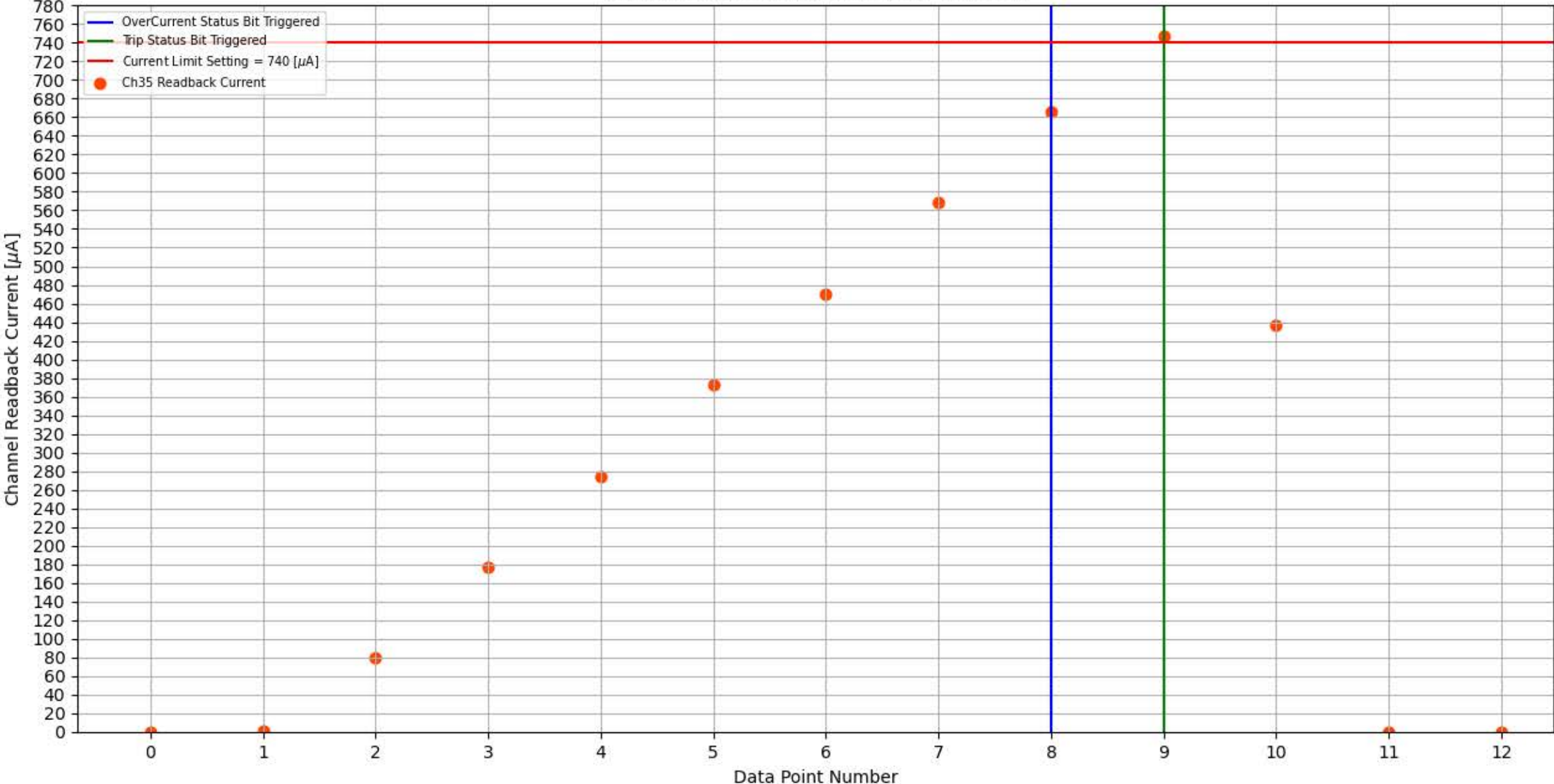
Module 256, Slot 3, Channel 35 Trip Test
