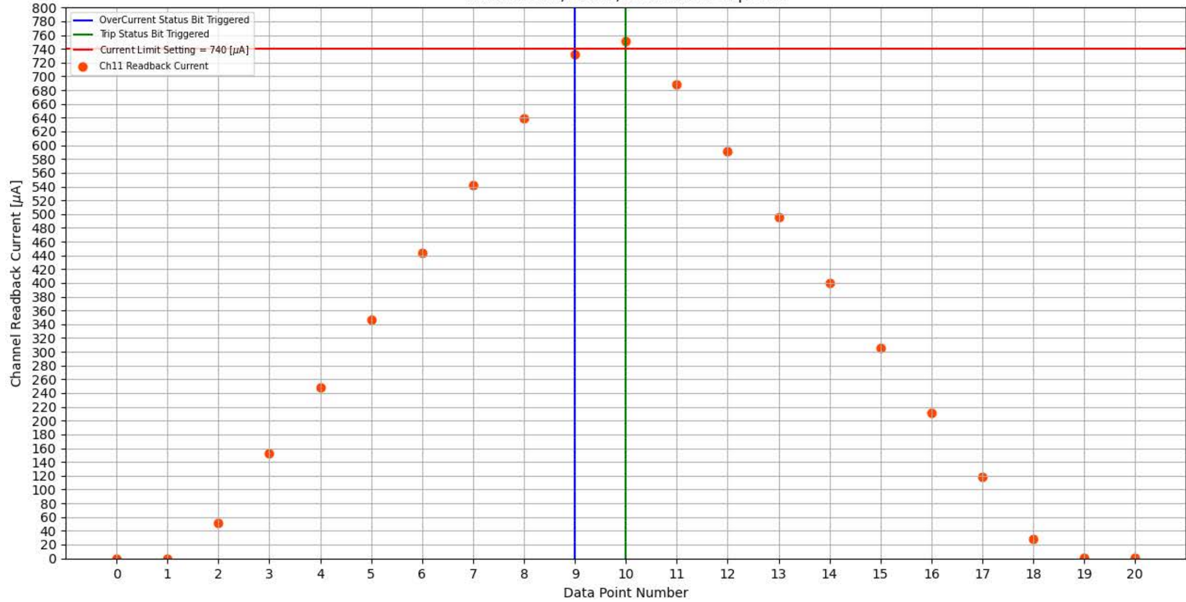
Module 256, Slot 3, Channel 11 Trip Test
