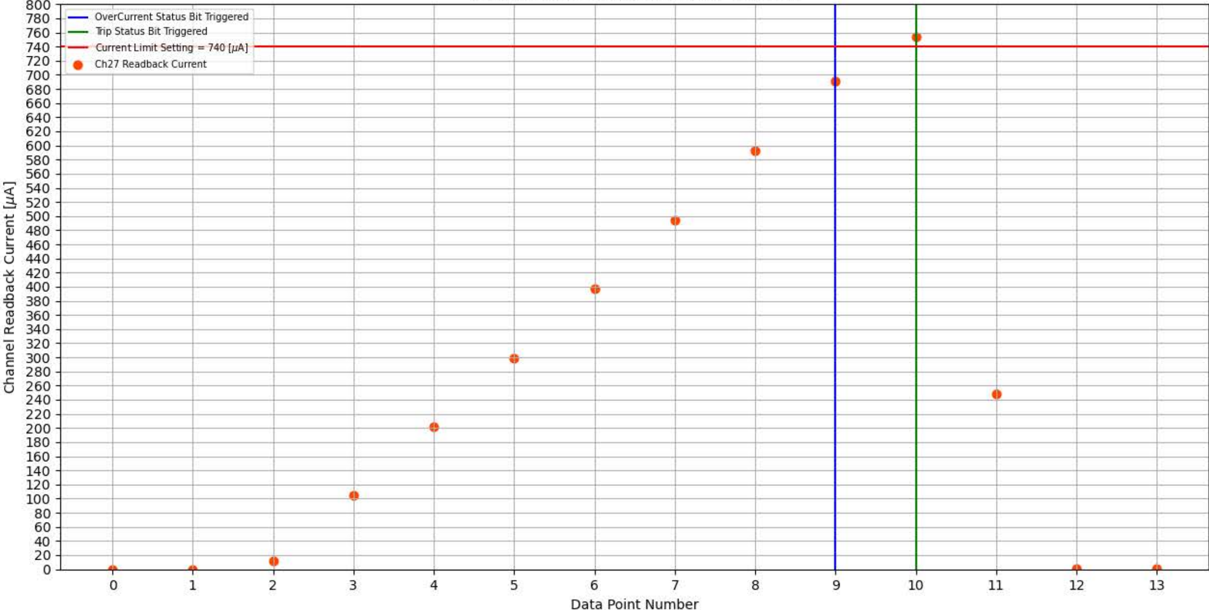
Module 256, Slot 3, Channel 27 Trip Test
