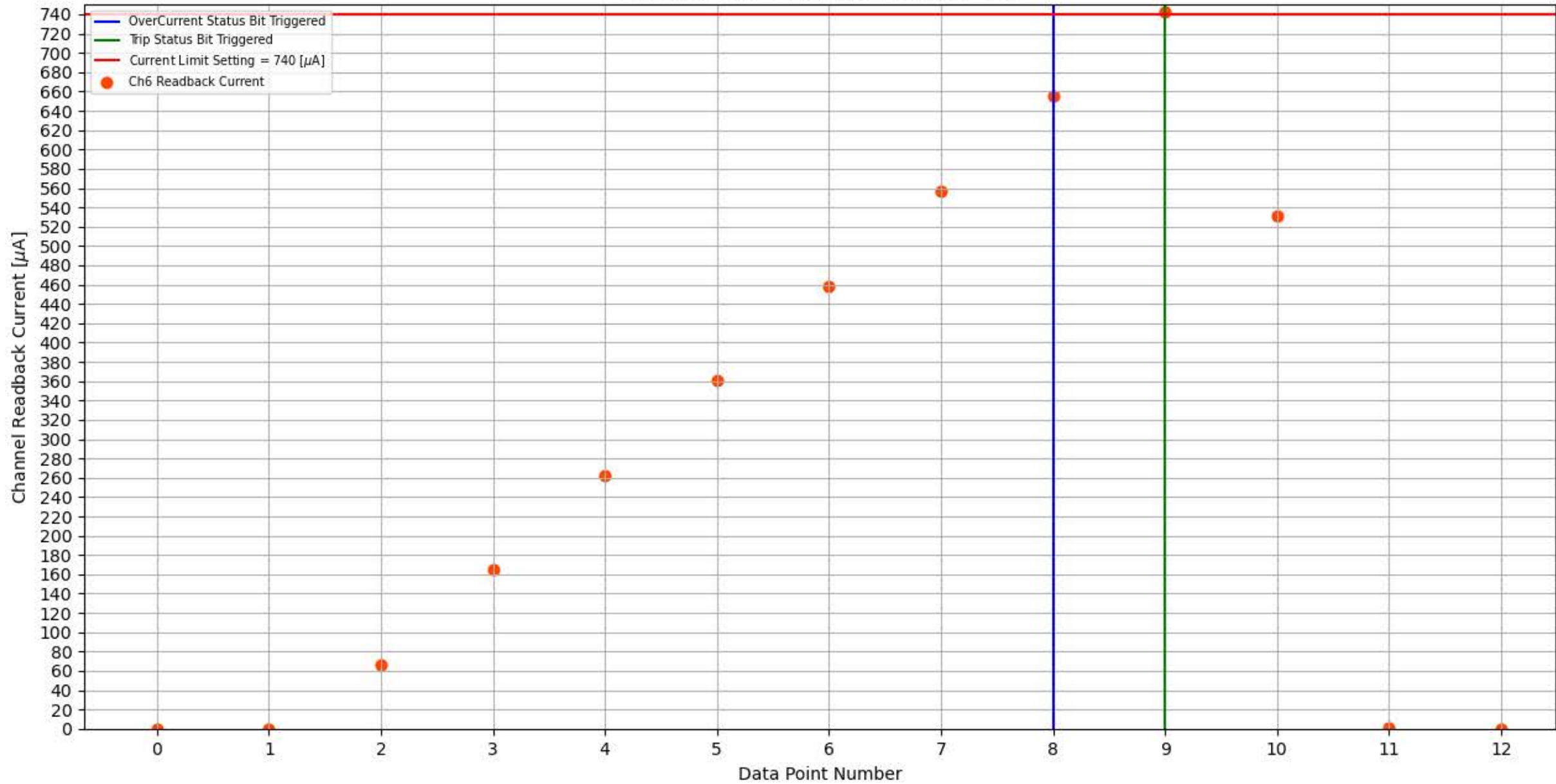
Module 256, Slot 3, Channel 6 Trip Test
