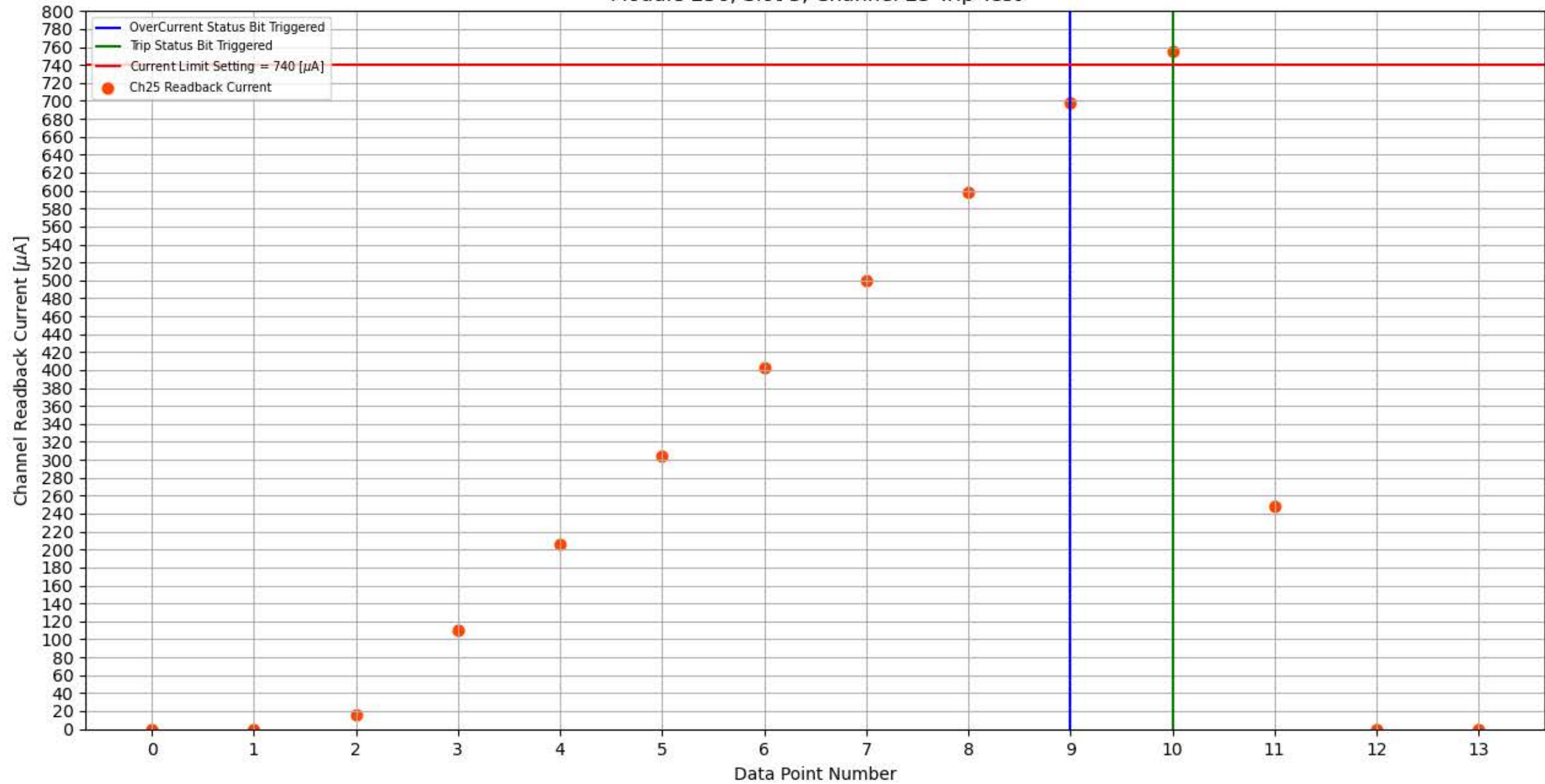
Module 256, Slot 3, Channel 25 Trip Test
