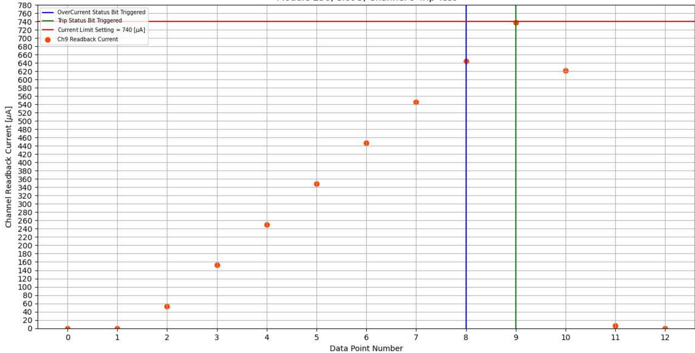
Module 256, Slot 3, Channel 9 Trip Test
