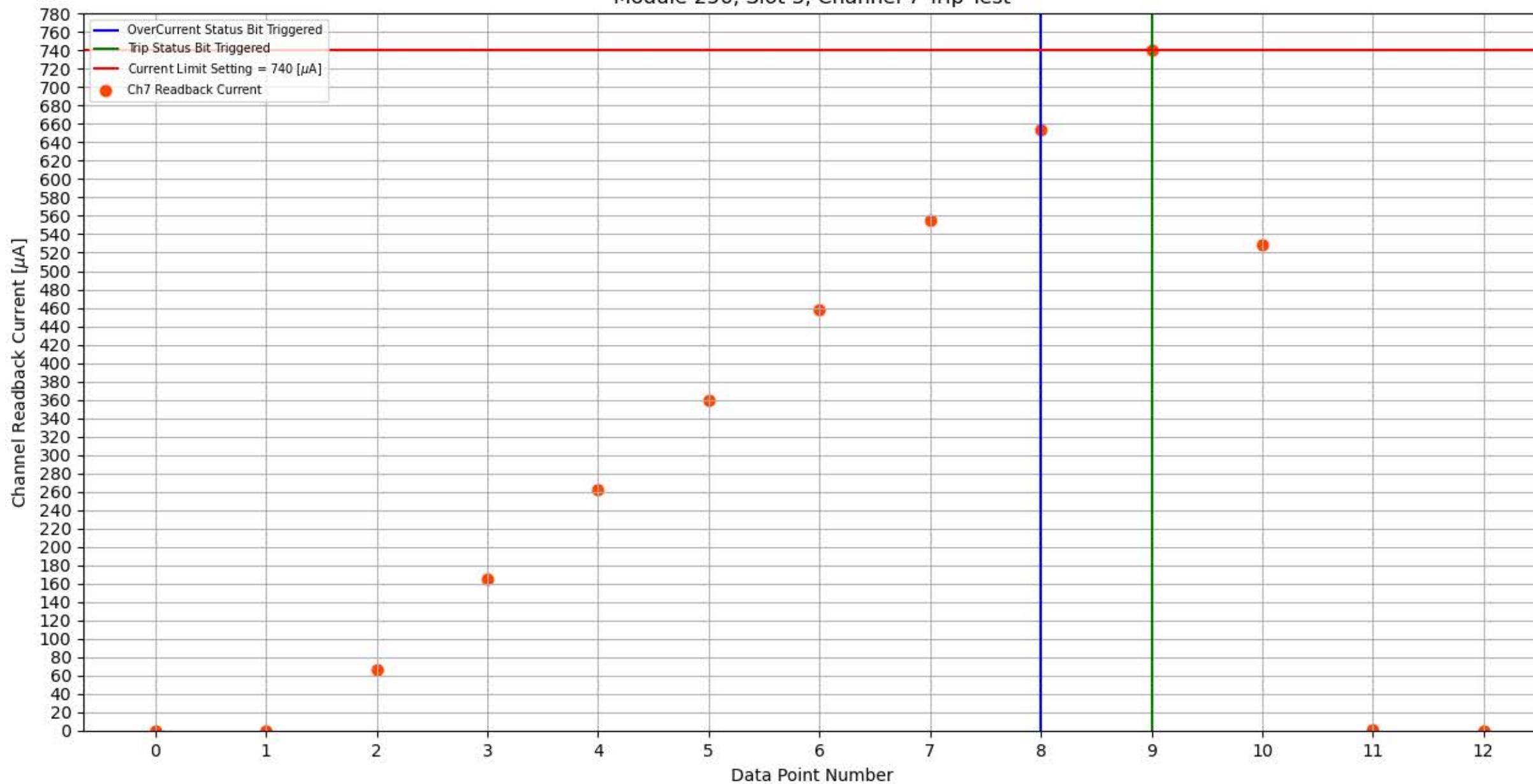
Module 256, Slot 3, Channel 7 Trip Test
