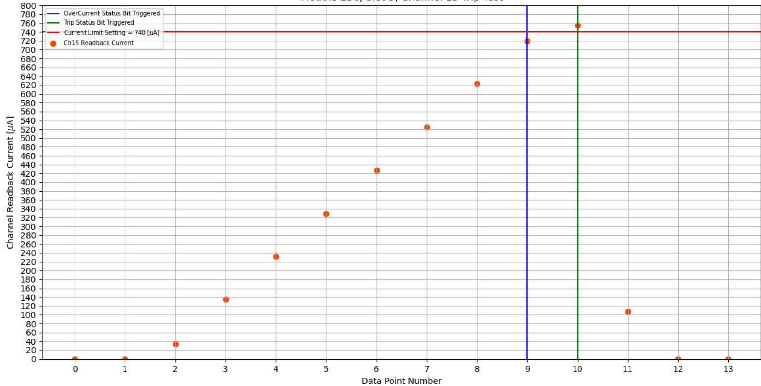
Module 256, Slot 3, Channel 15 Trip Test
