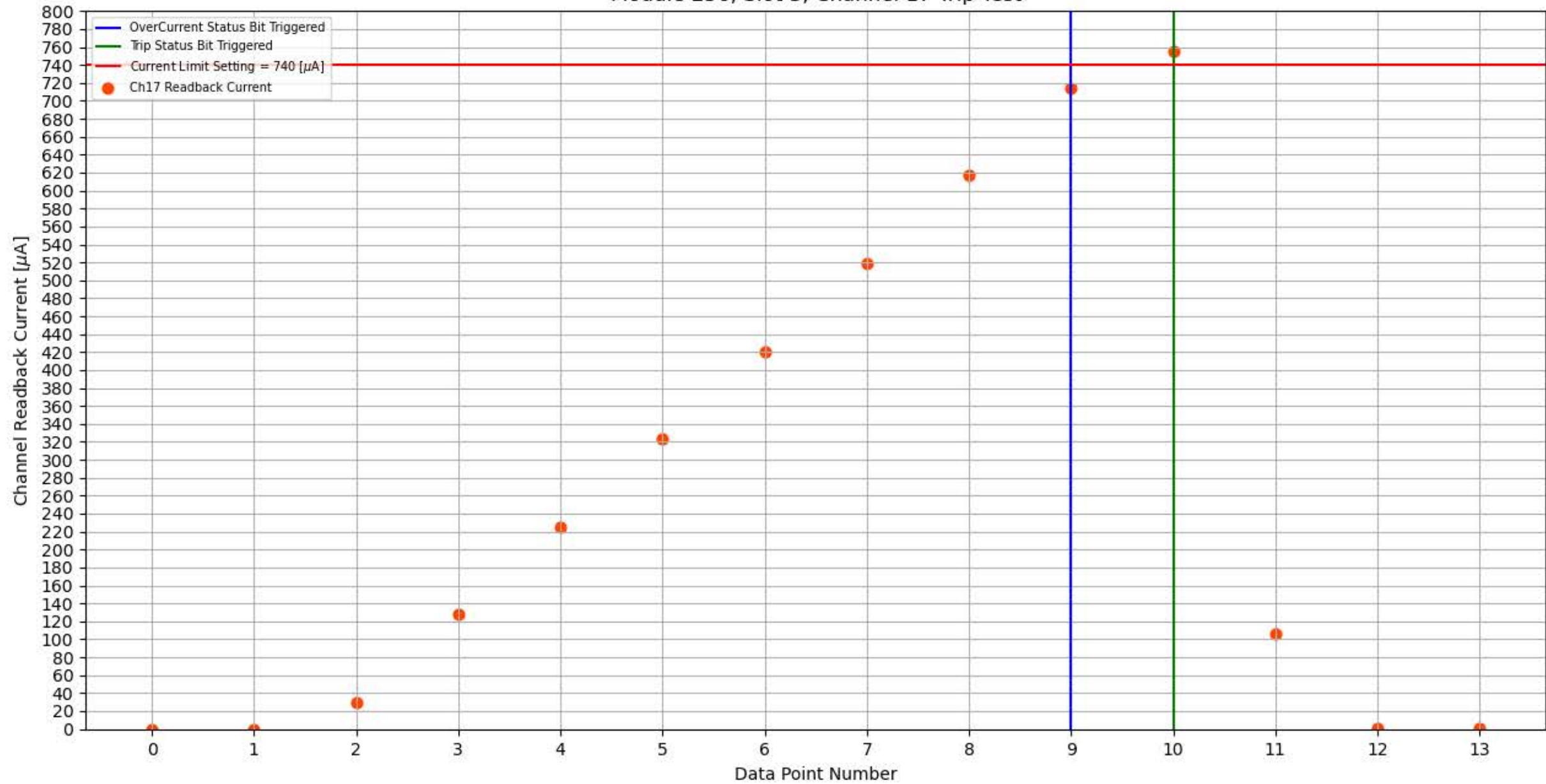
Module 256, Slot 3, Channel 17 Trip Test
