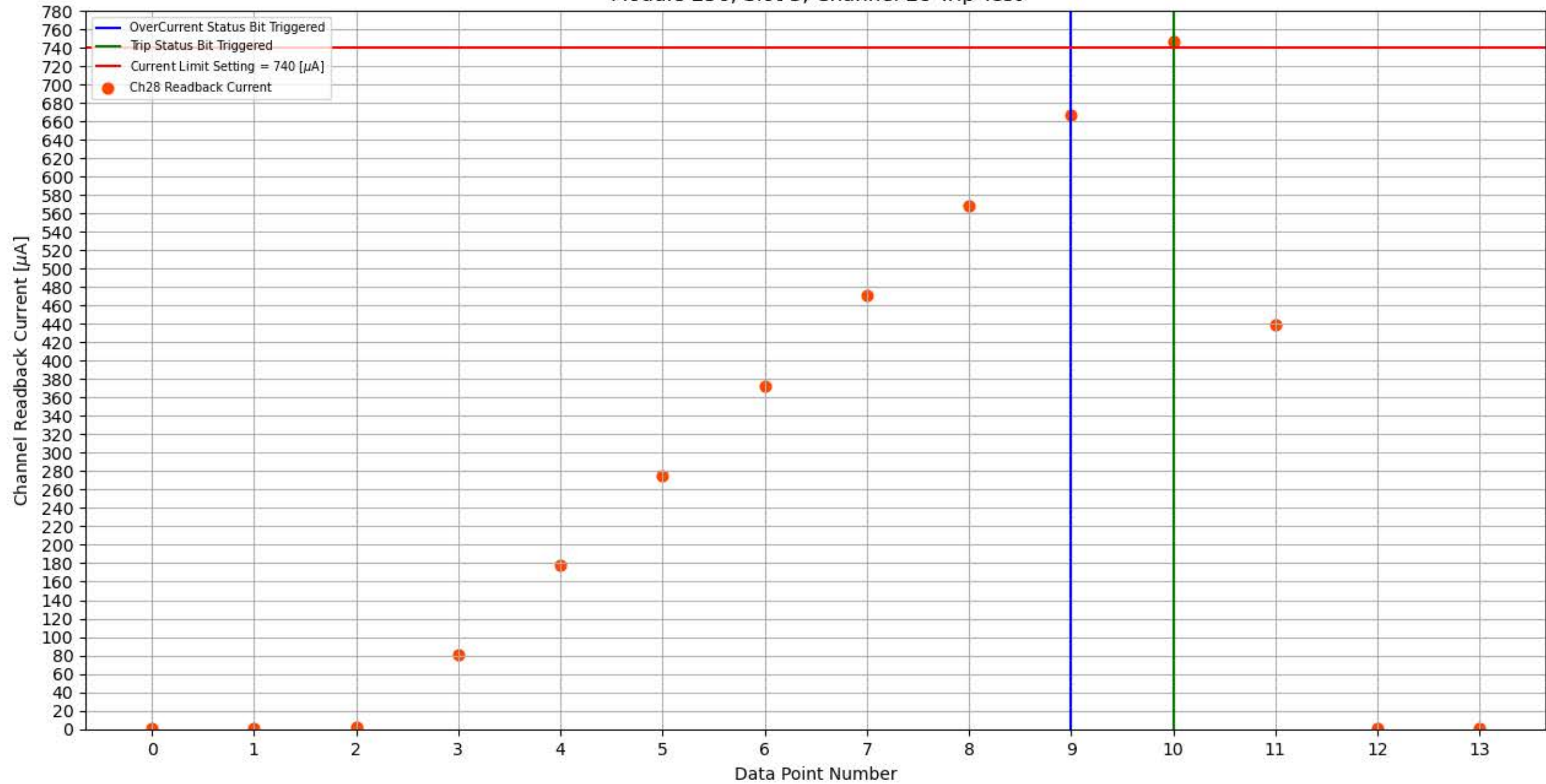
Module 256, Slot 3, Channel 28 Trip Test
