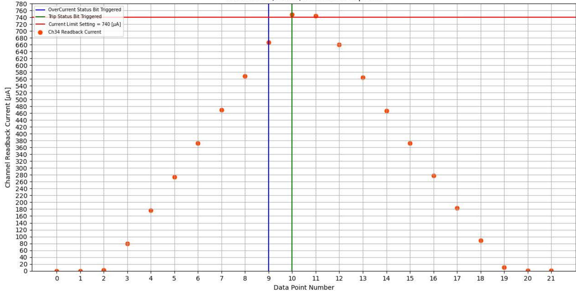
Module 256, Slot 3, Channel 34 Trip Test
