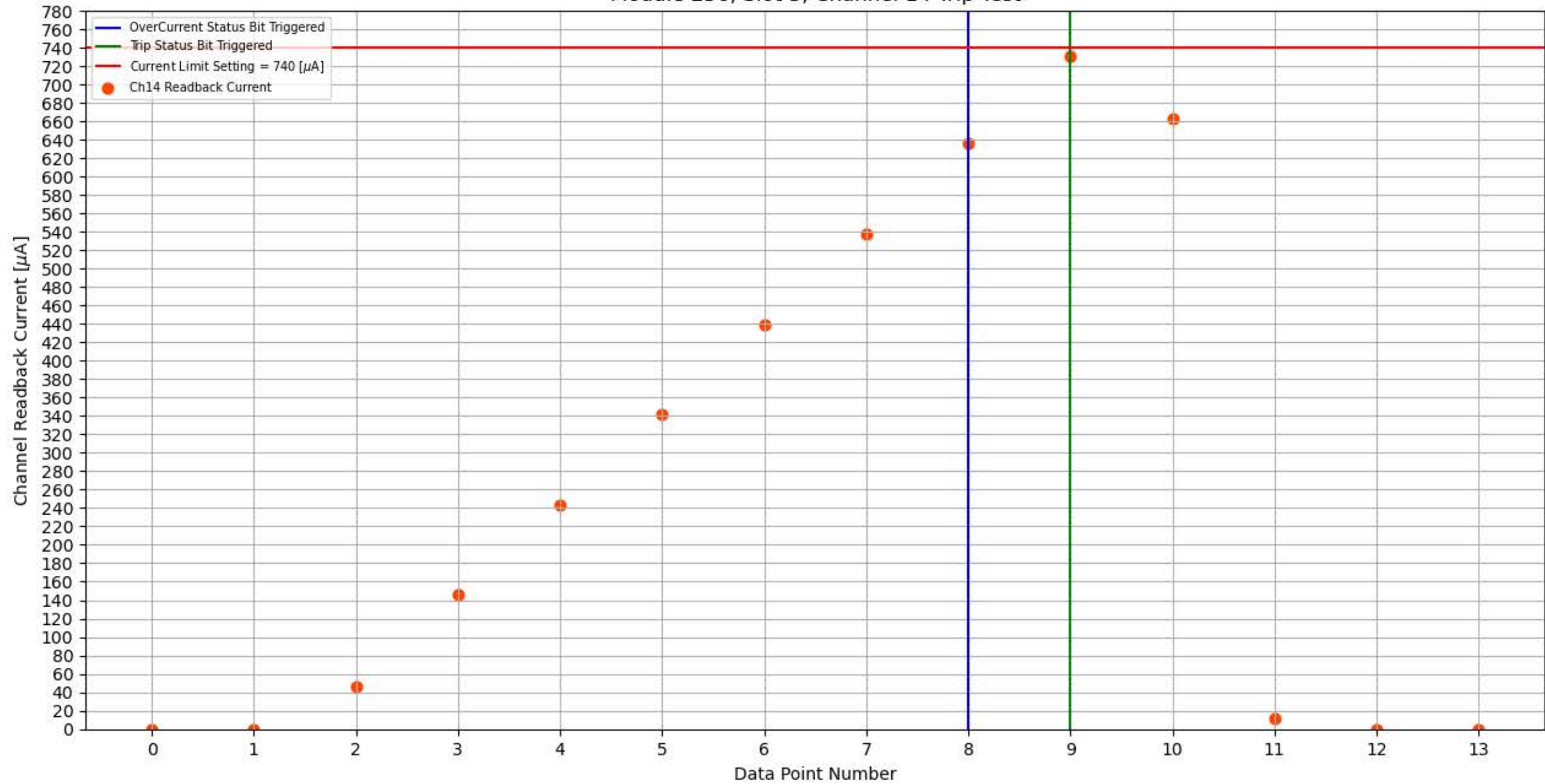
Module 256, Slot 3, Channel 14 Trip Test
