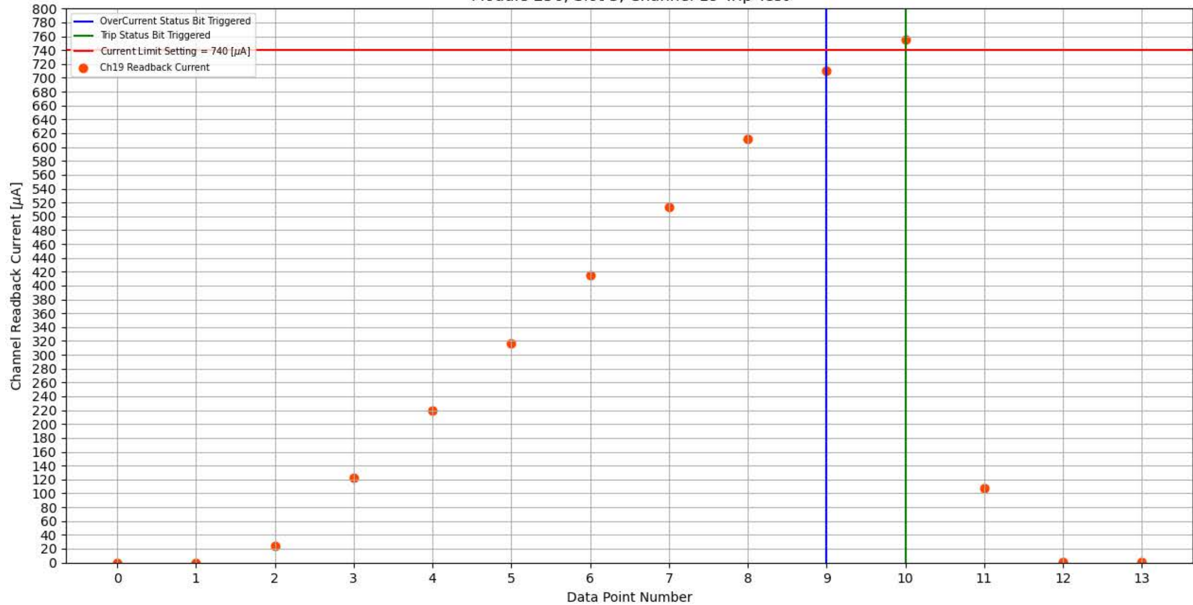
Module 256, Slot 3, Channel 19 Trip Test
