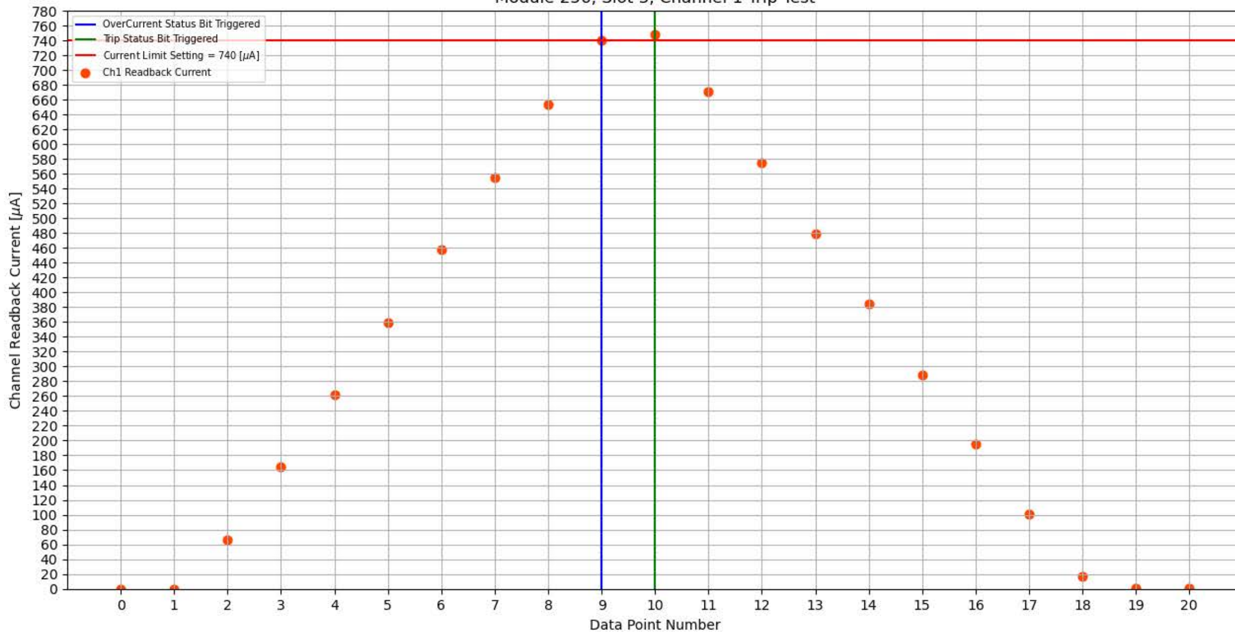
Module 256, Slot 3, Channel 1 Trip Test
