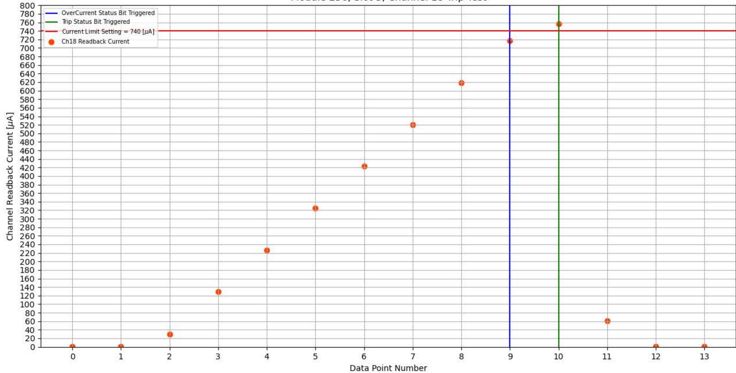
Module 256, Slot 3, Channel 18 Trip Test
