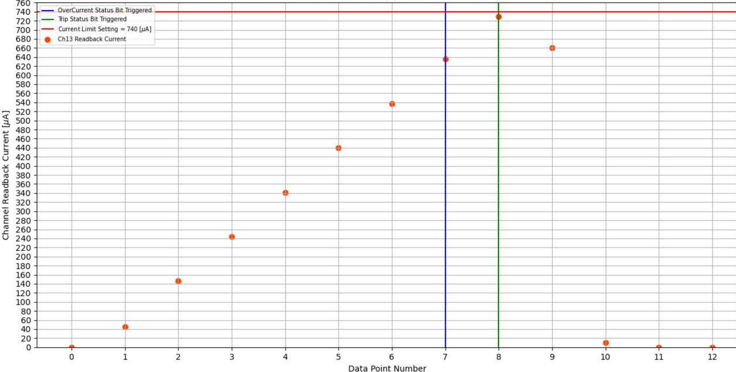
Module 256, Slot 3, Channel 13 Trip Test
