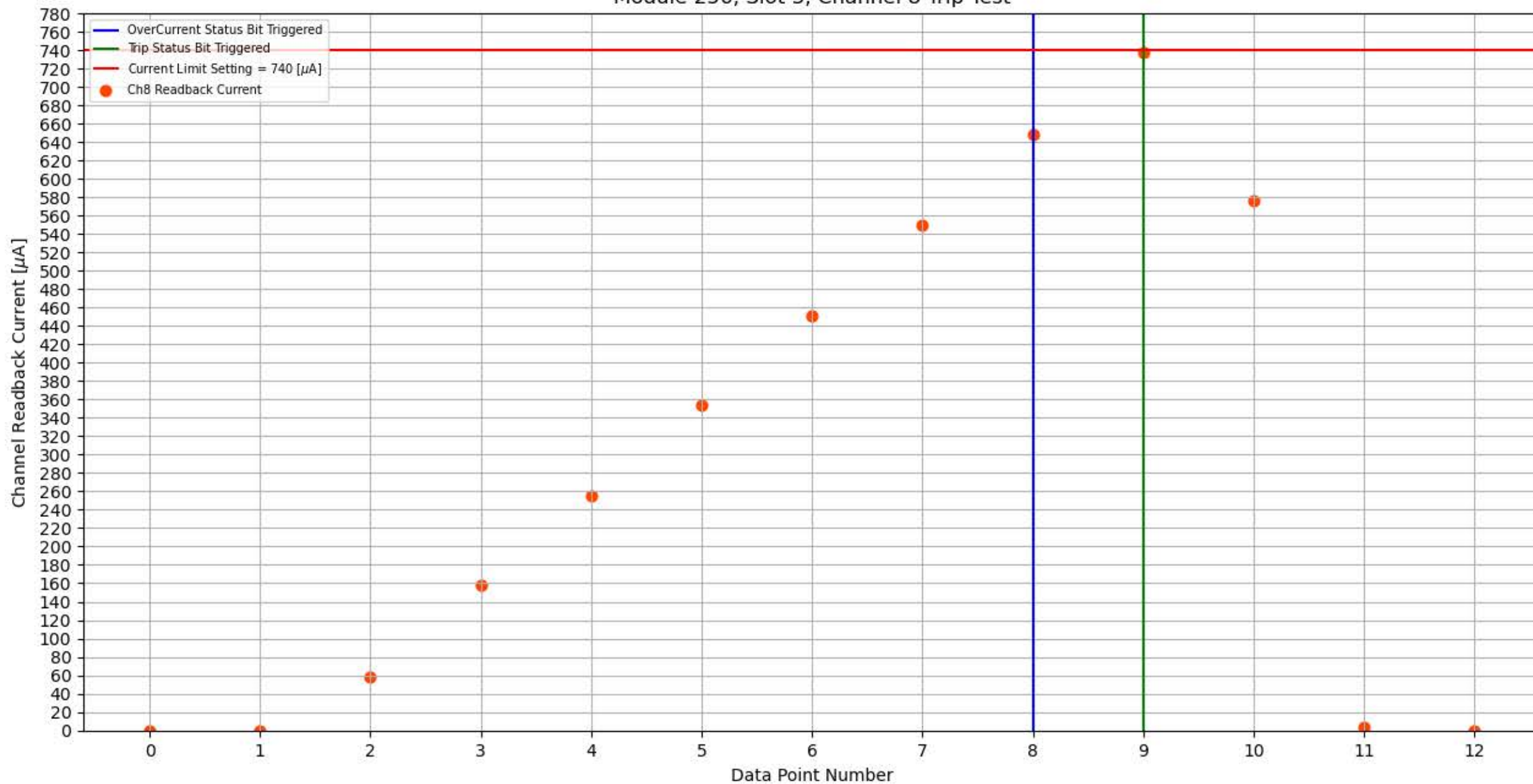
Module 256, Slot 3, Channel 8 Trip Test
