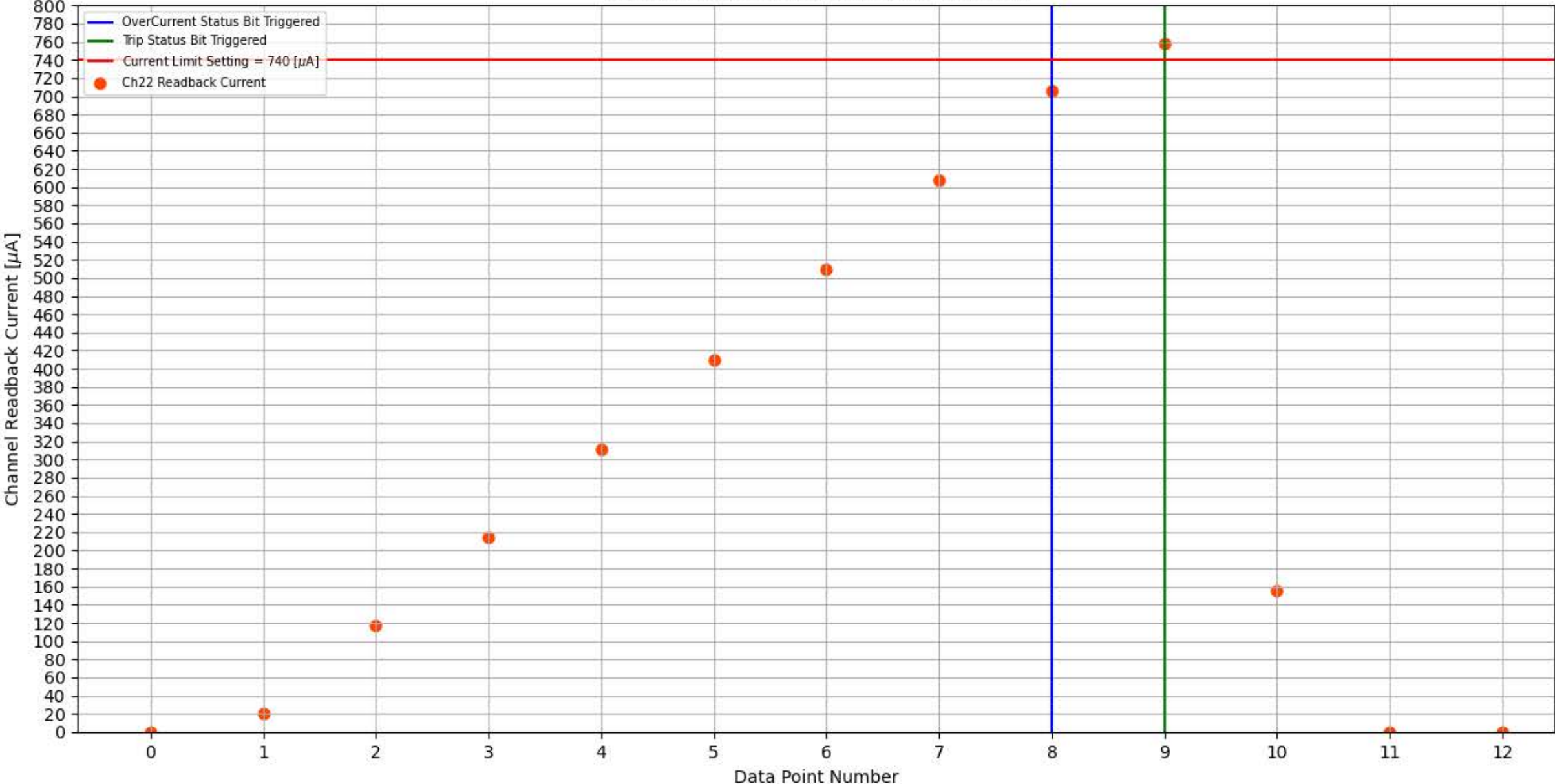
Module 256, Slot 3, Channel 22 Trip Test
