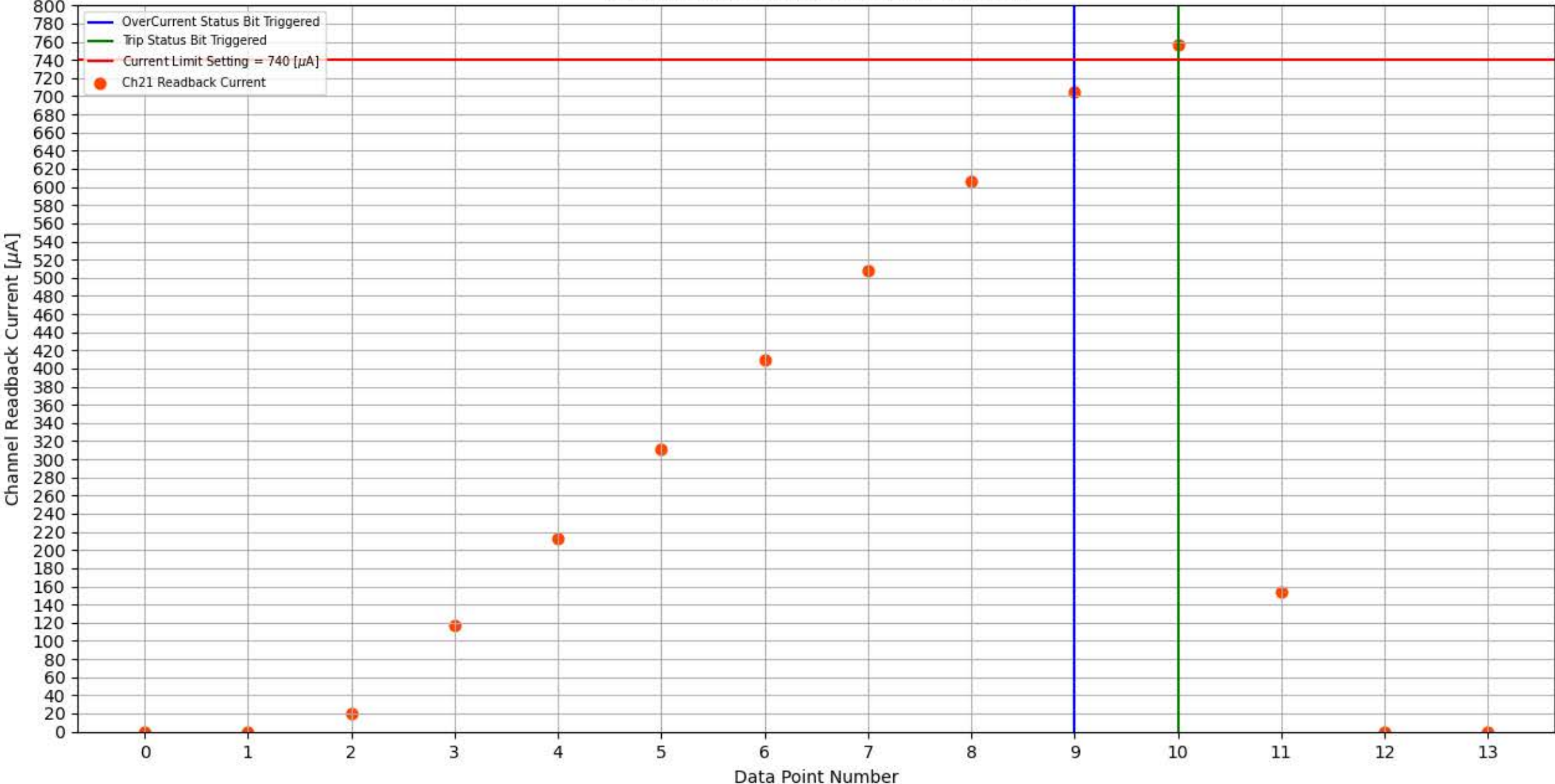
Module 256, Slot 3, Channel 21 Trip Test
