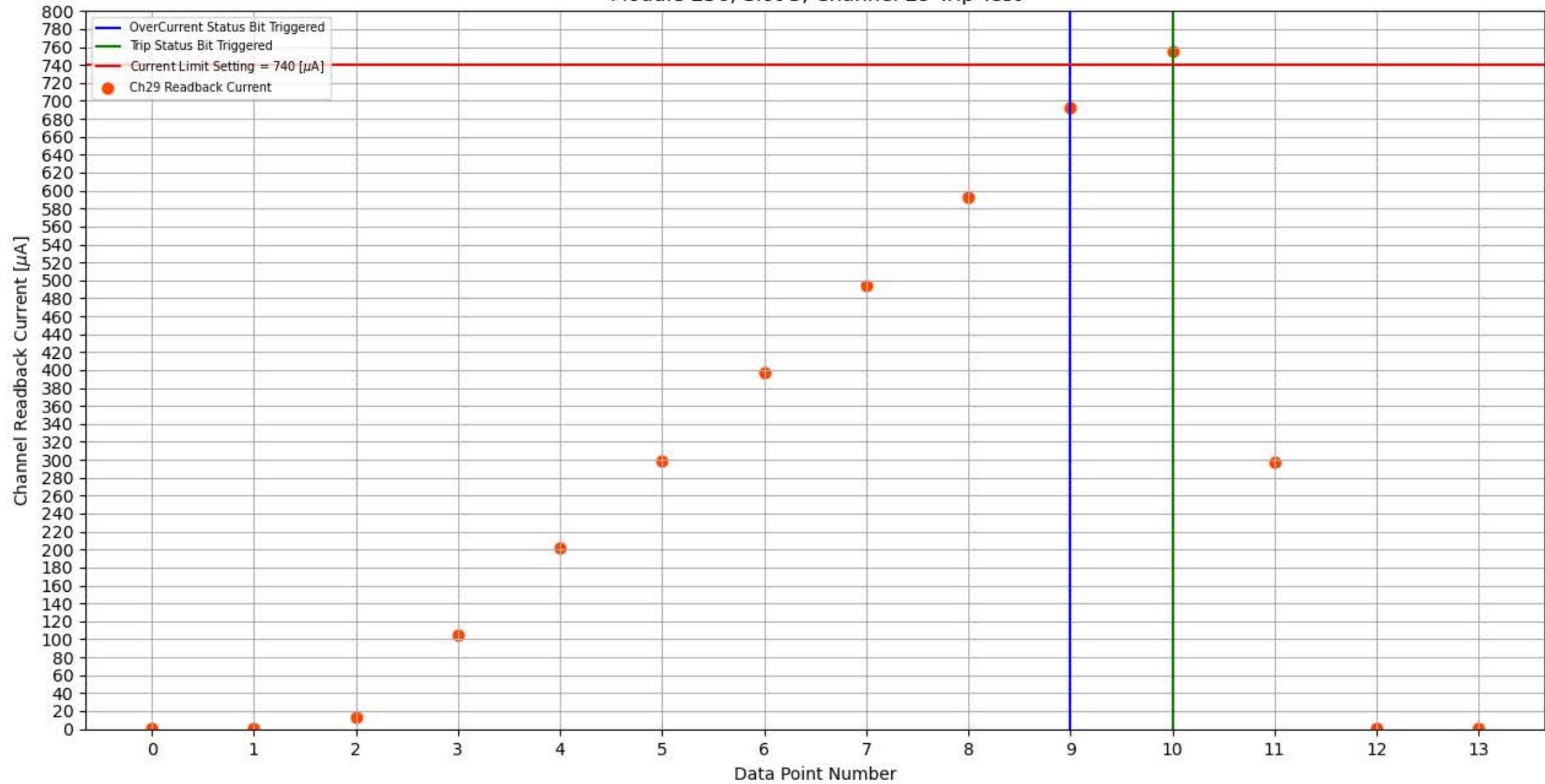
Module 256, Slot 3, Channel 29 Trip Test
