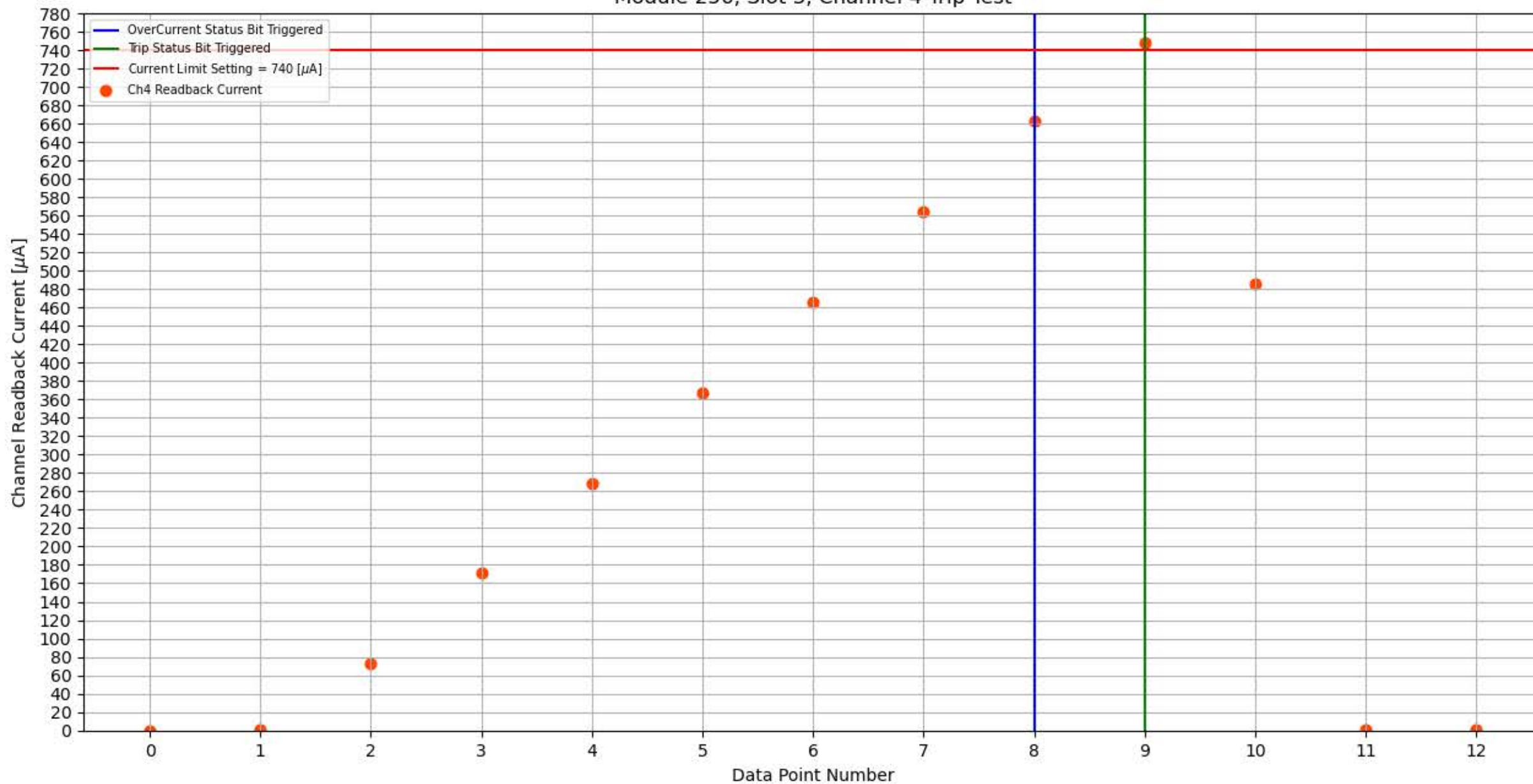
Module 256, Slot 3, Channel 4 Trip Test
