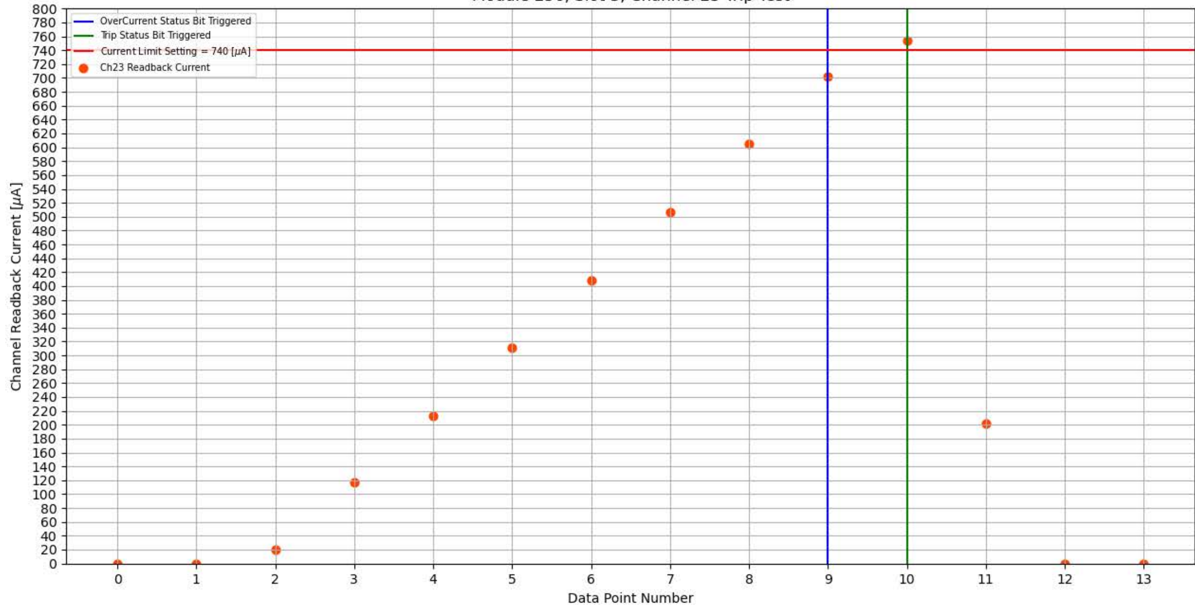
Module 256, Slot 3, Channel 23 Trip Test
