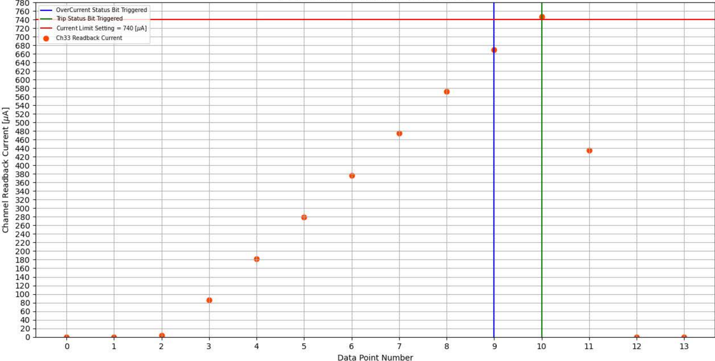
Module 256, Slot 3, Channel 33 Trip Test
