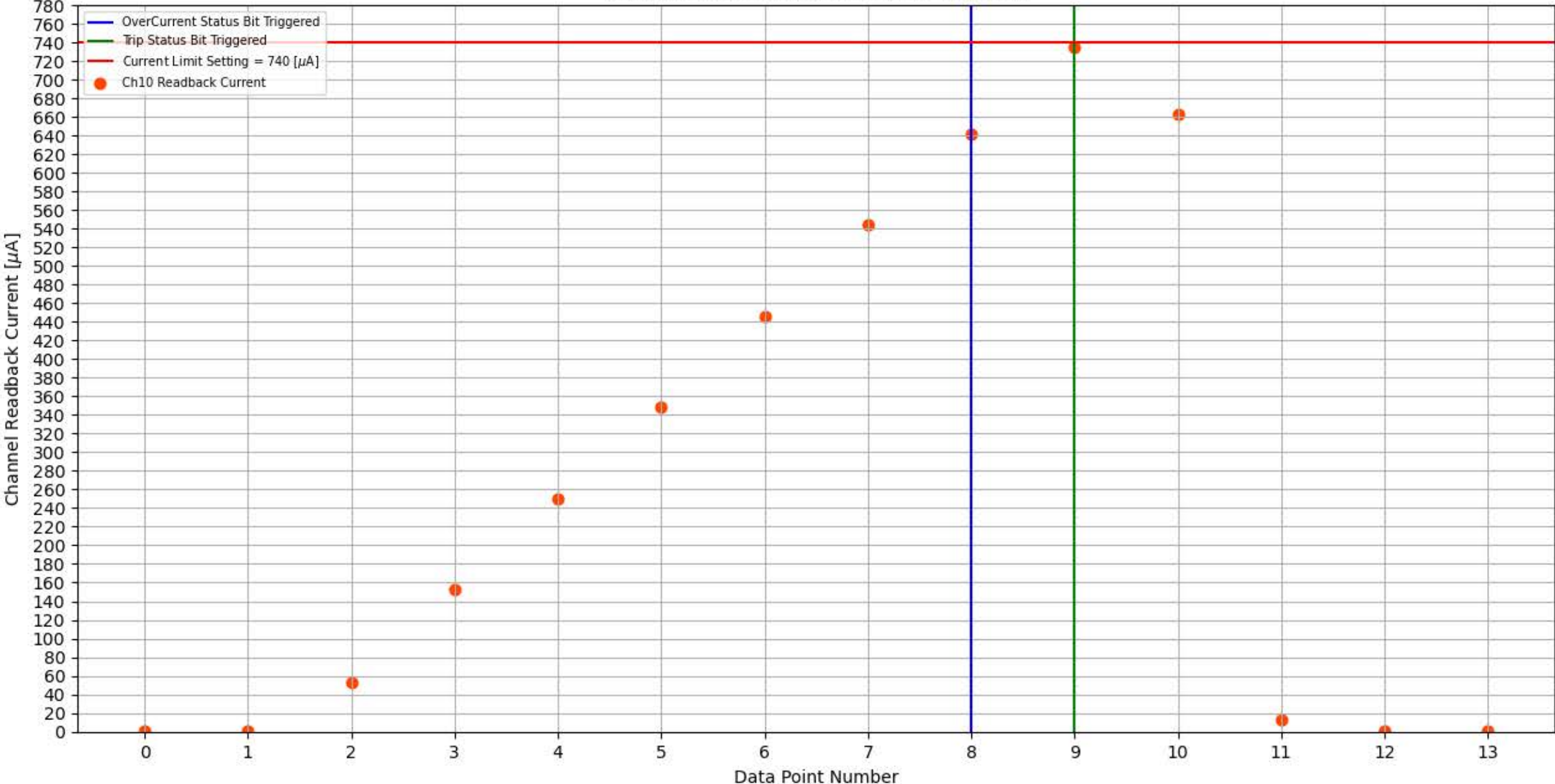
Module 256, Slot 3, Channel 10 Trip Test
