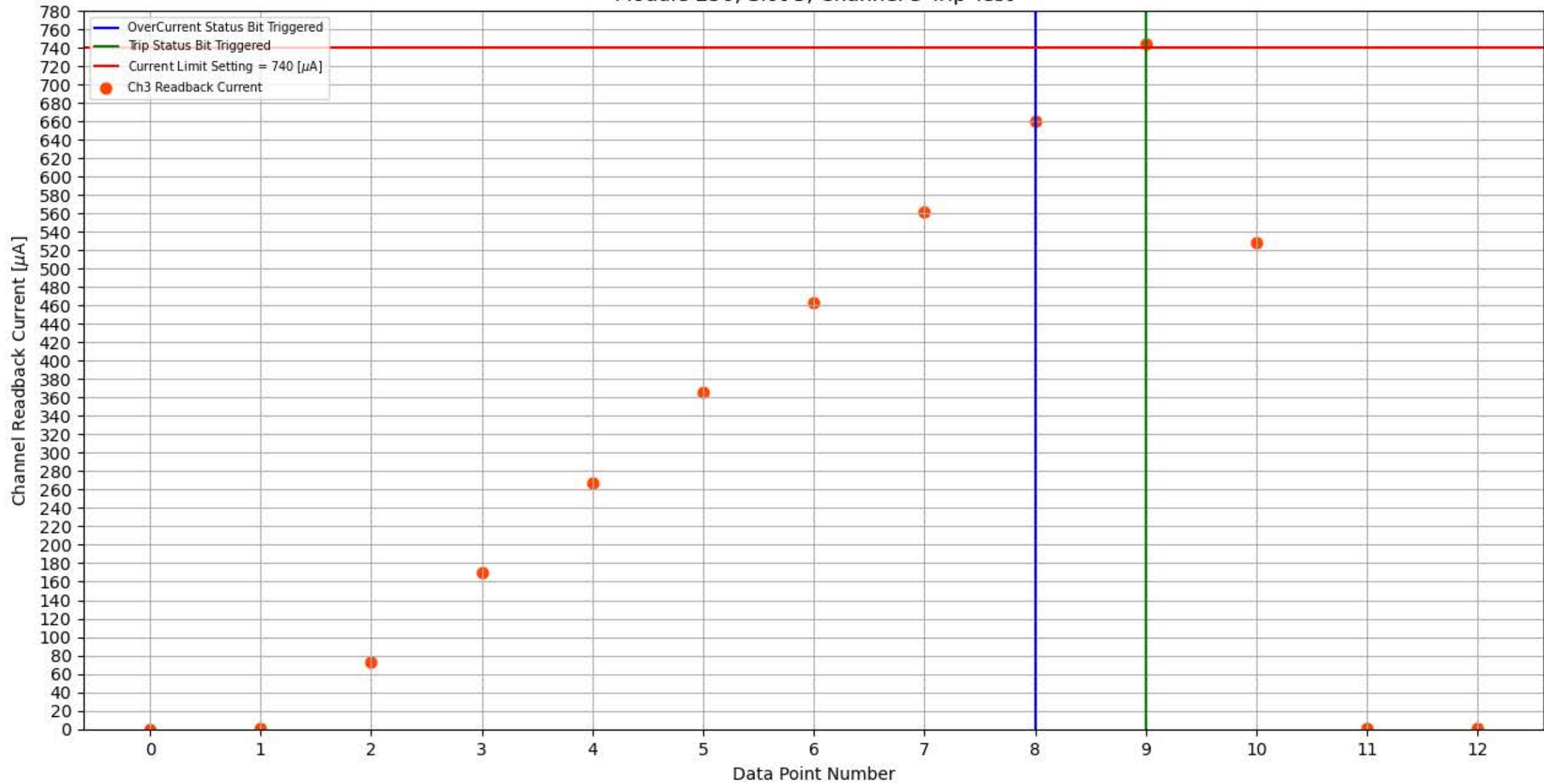
Module 256, Slot 3, Channel 3 Trip Test
